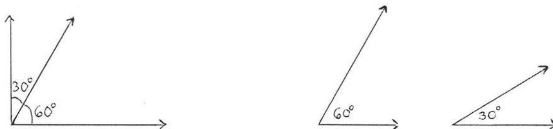
Figure 5. Complementary angles.
