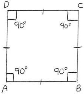
Figure 9. A square.
