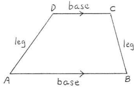
Figure 10. A trapezoid.
