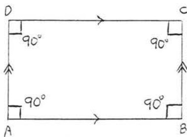
Figure 5. A rectangle.
